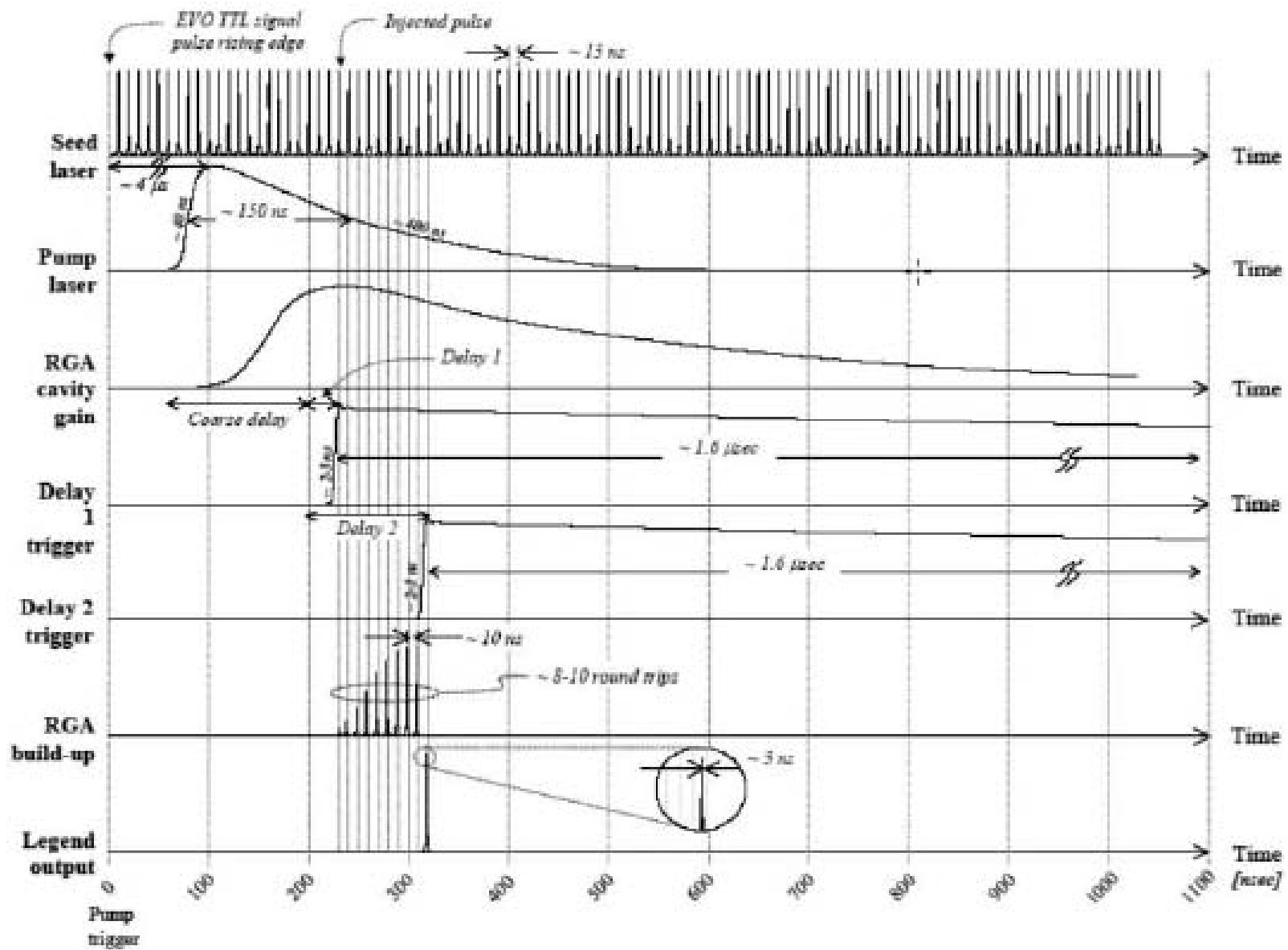
Timing diagram of the laser system
