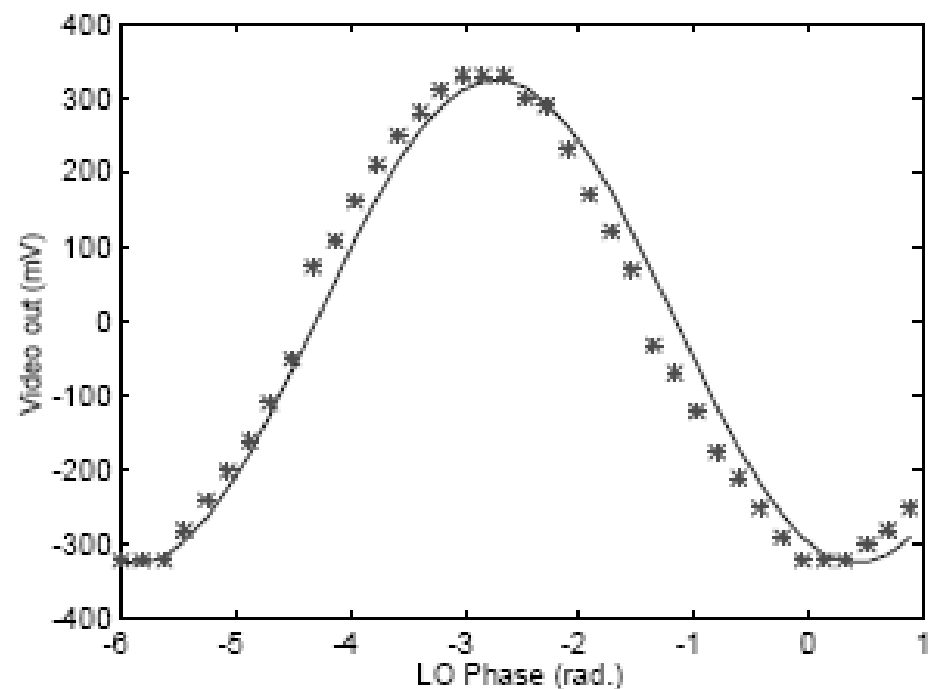
Figure 5. Stripline BPM sum video out vs. Local oscillator phase.
