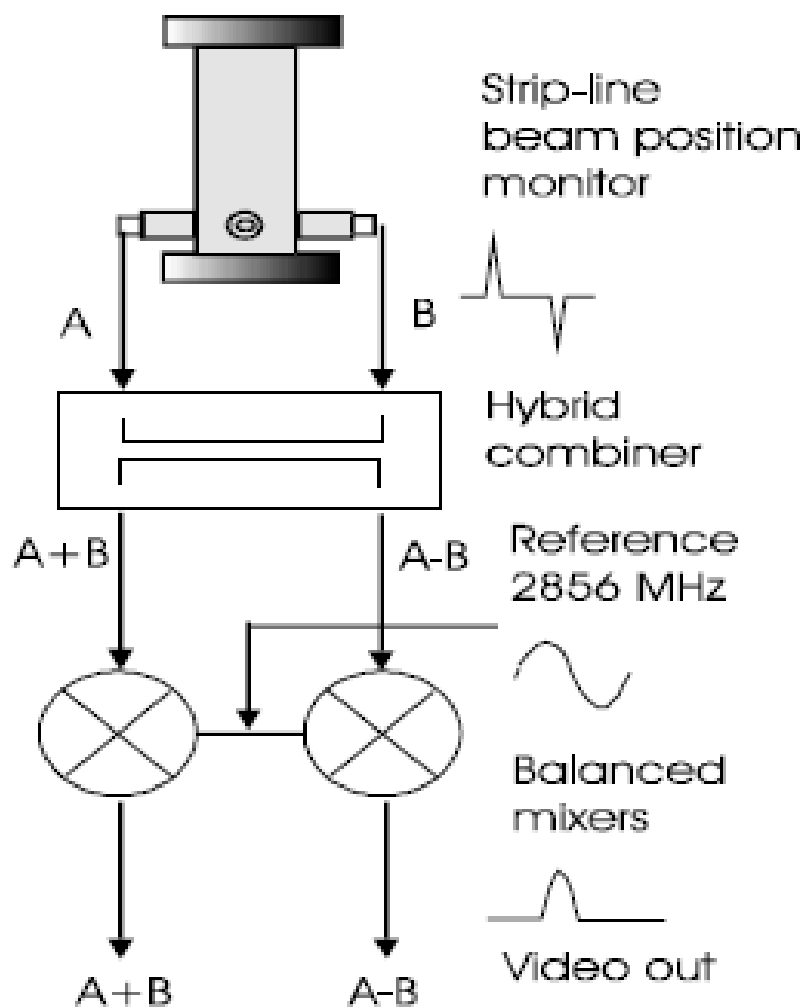
Figure 1. The stripline beam position monitor system.
