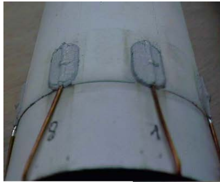
Thermal-Sprayed Heaters
