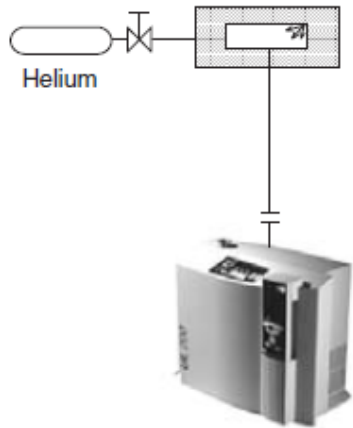
a: Integral leak detection; vacuum inside specimen
