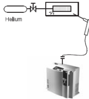
c: Integral leak detection (test gas enrichment inside the enclosure); pressurized test gas inside specimen
