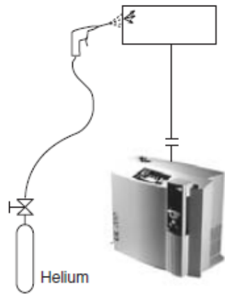
b: Local leak detection; vacuum inside specimen
